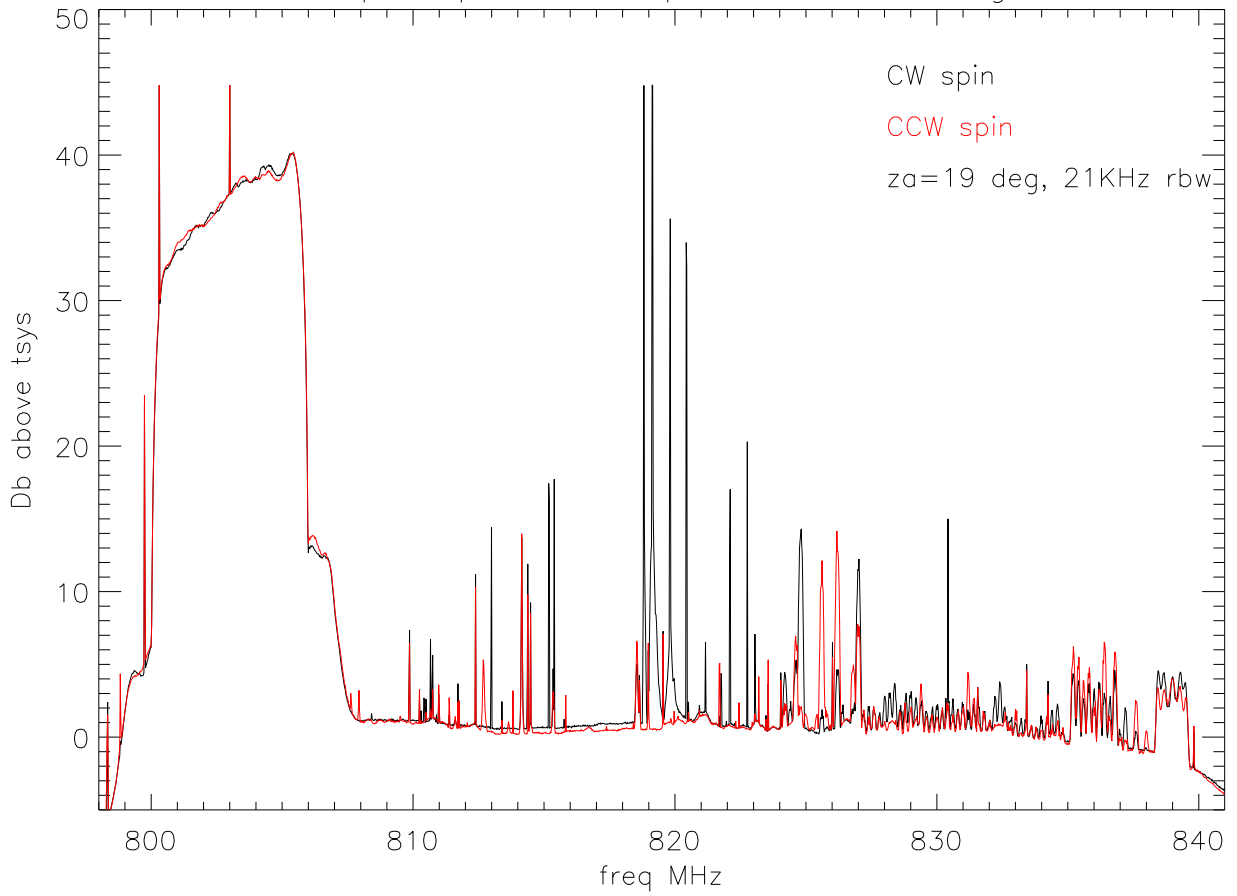
13apr09 Average spectra value for az swings
