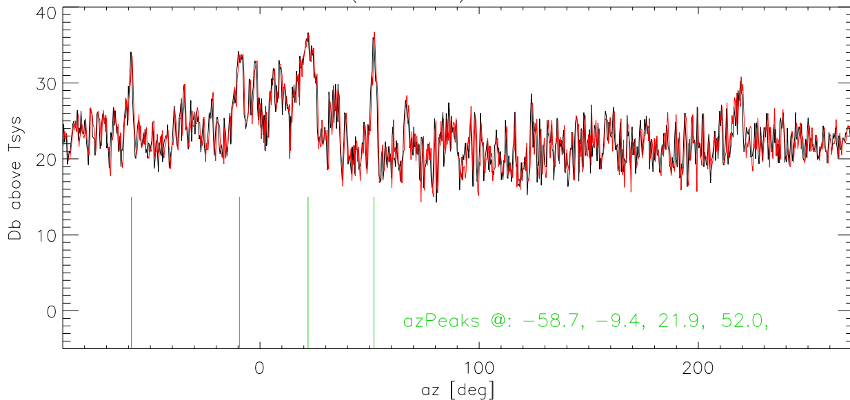
818.81 birdie strength vs az (rbw=21Khz)
