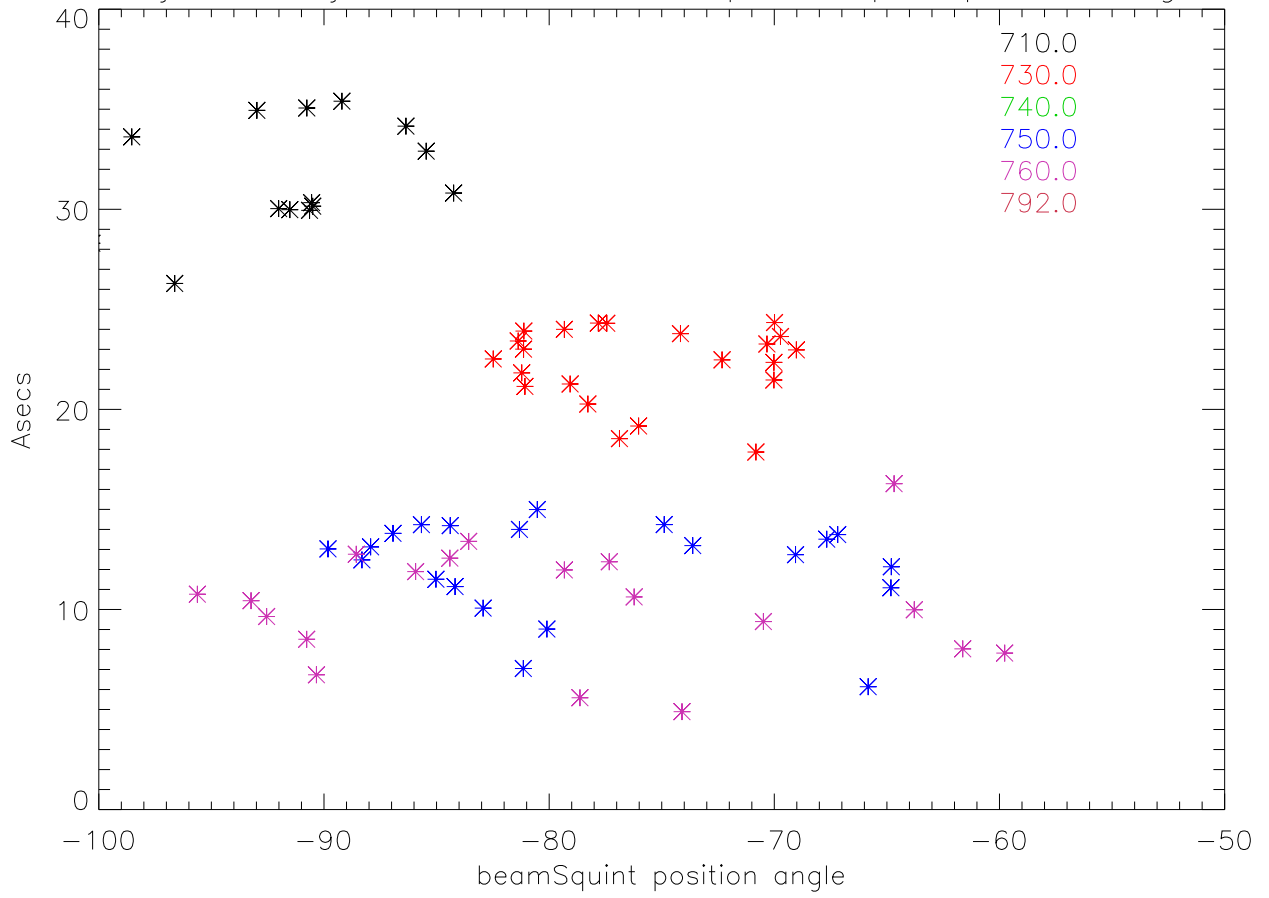
28jun09-02jul09 800Mhz beam squint amp vs position angle
