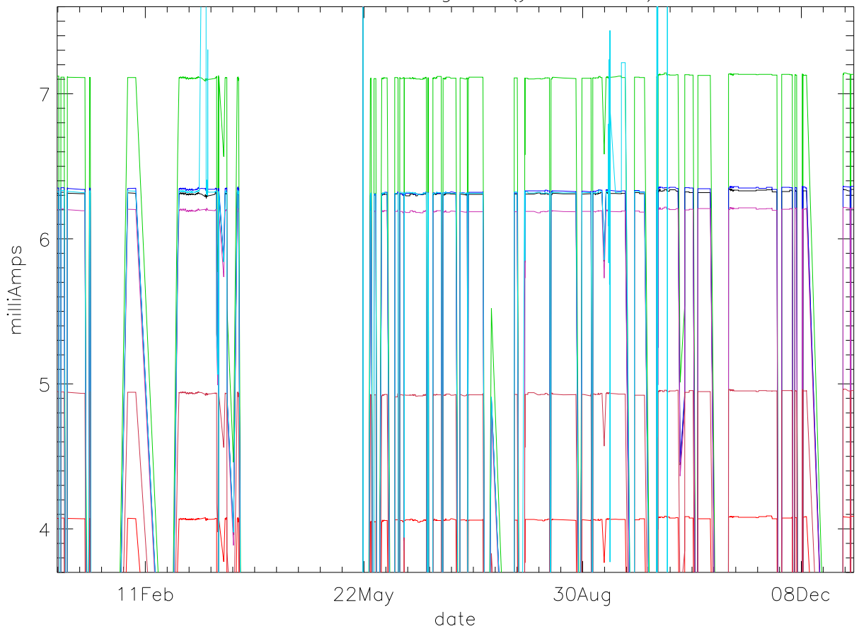
Id:Drain Current. stage 1 (year 2014) PoIB
