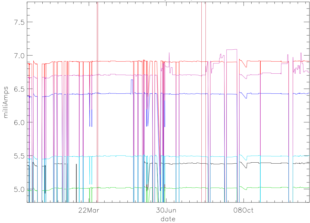
Id:Drain Current. stage 2 (year 2018) PoIB
