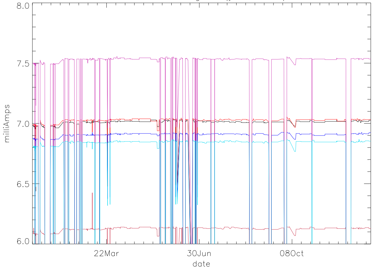
Id:Drain Current. stage 3 (year 2018) PoIB
