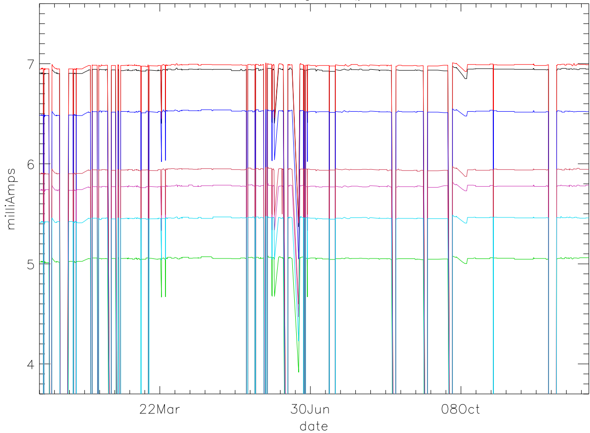
Id:Drain Current. stage 1 (year 2018) PoIB
