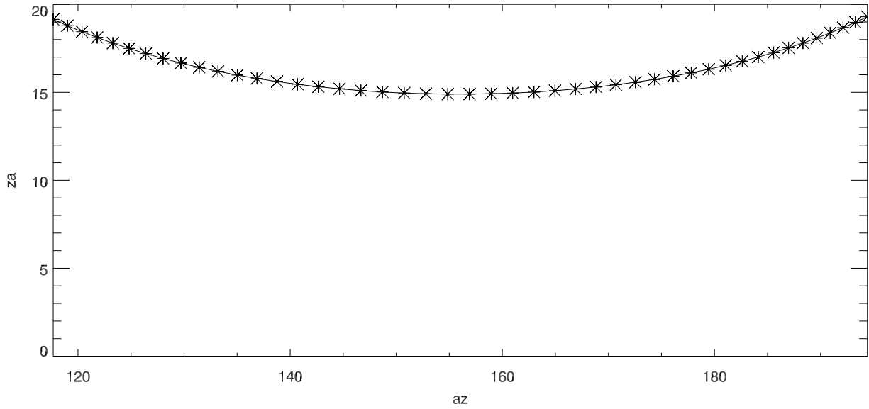
2018cb az,za track for 09feb18
