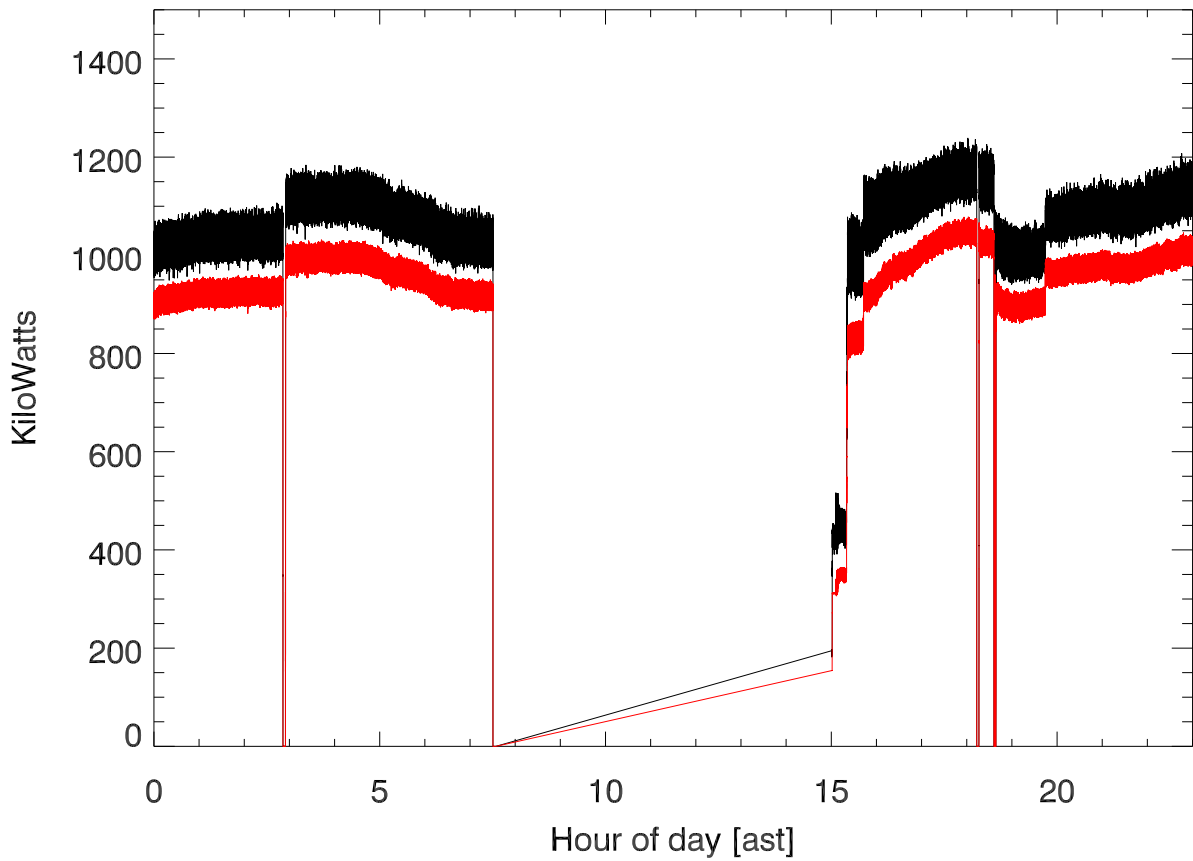
20180116 T1193 430tx power (dome) vs hour of day
