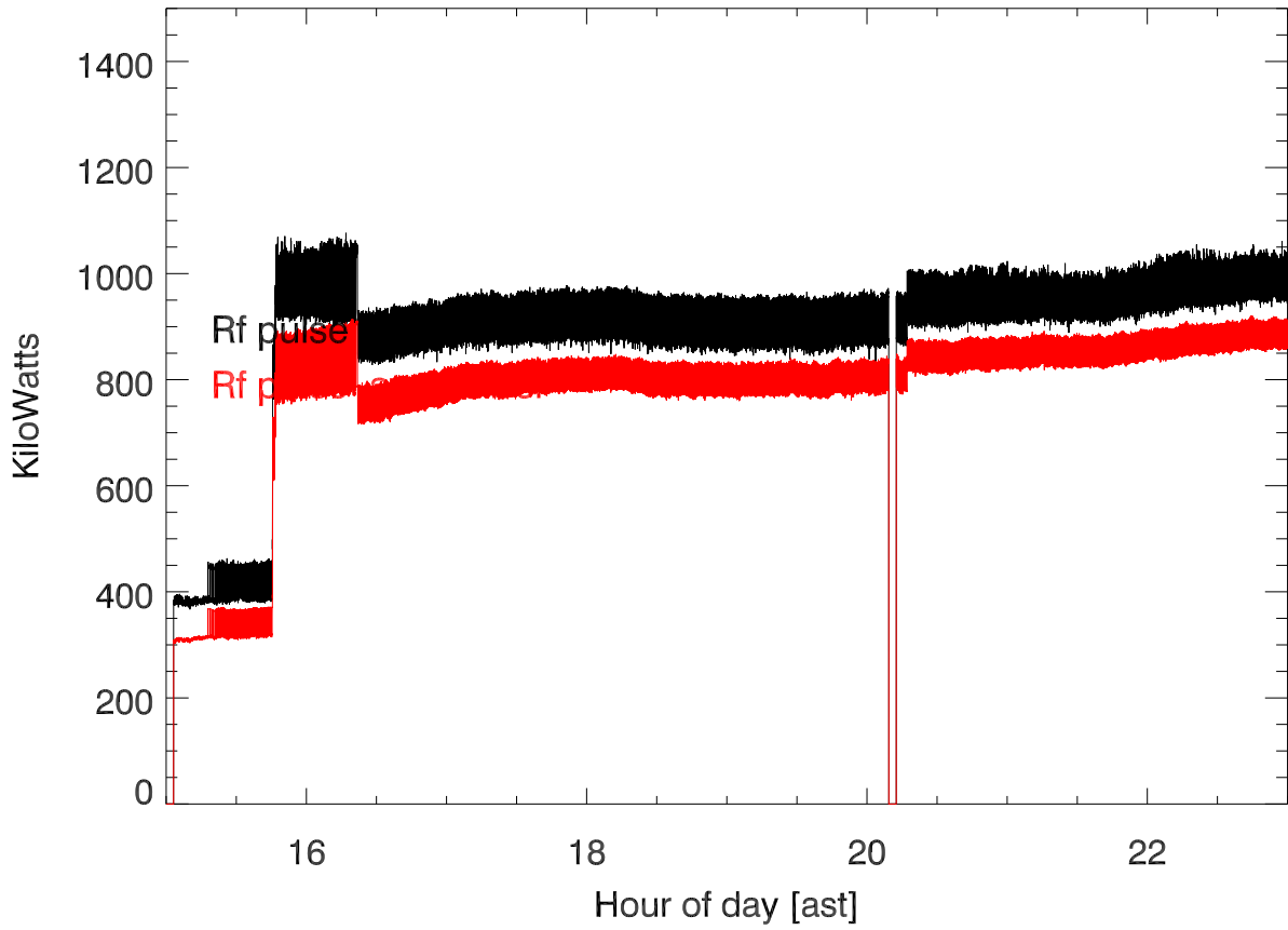
20180115 T1193 430tx power (dome) vs hour of day
