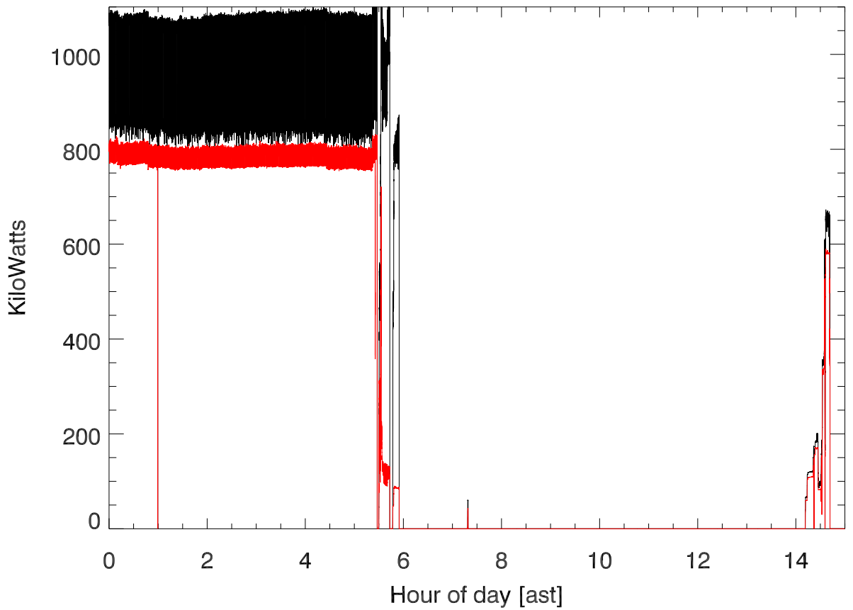
20191012 T3364 430tx power (dome) vs hour of day
