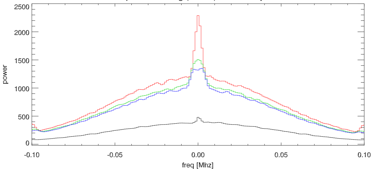
04apr14 t2867 avg (30 sec) decoded spectra
