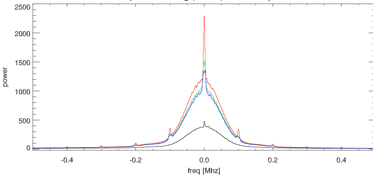
04apr14 t2867 avg (30 sec) decoded spectra
