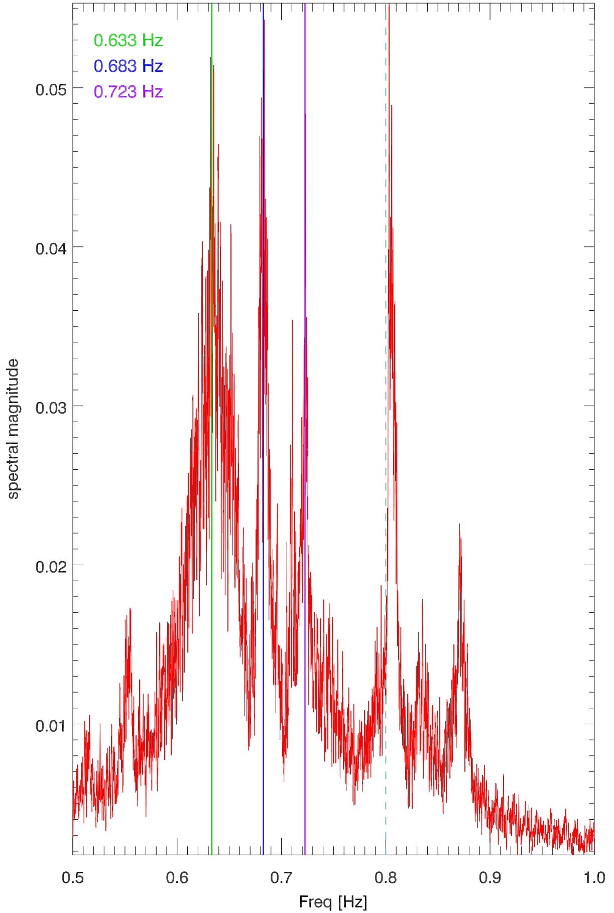
blowup of spectra 22.0 to 22.2 hours
