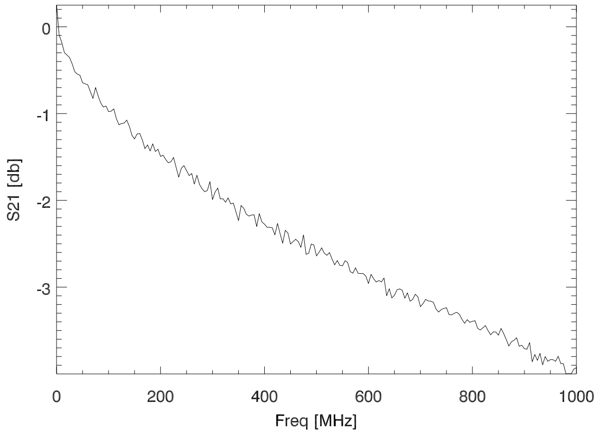
210422 S21 (cable loss) for discone measurement at 12m
