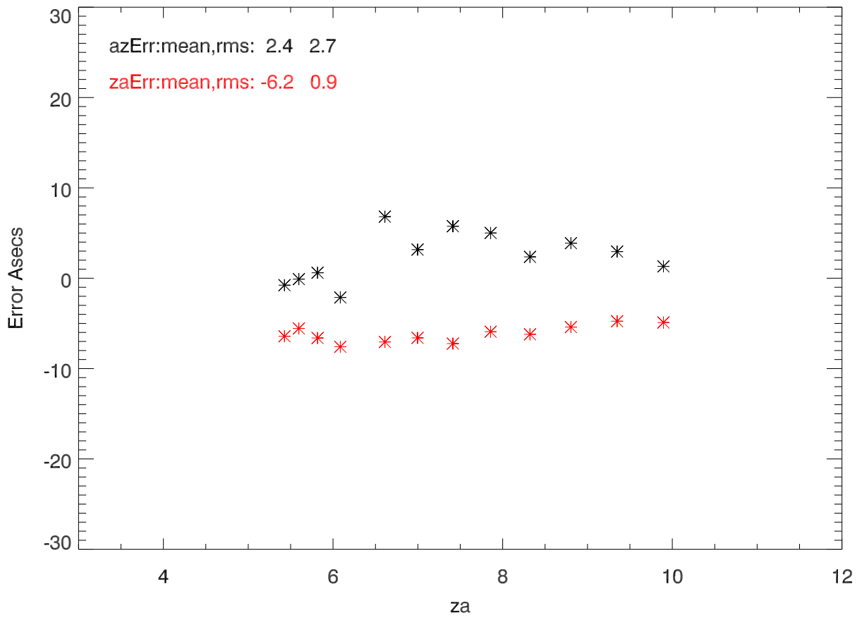
dipole 0 Position A0 cross scan pointing err vs za 14jun10
