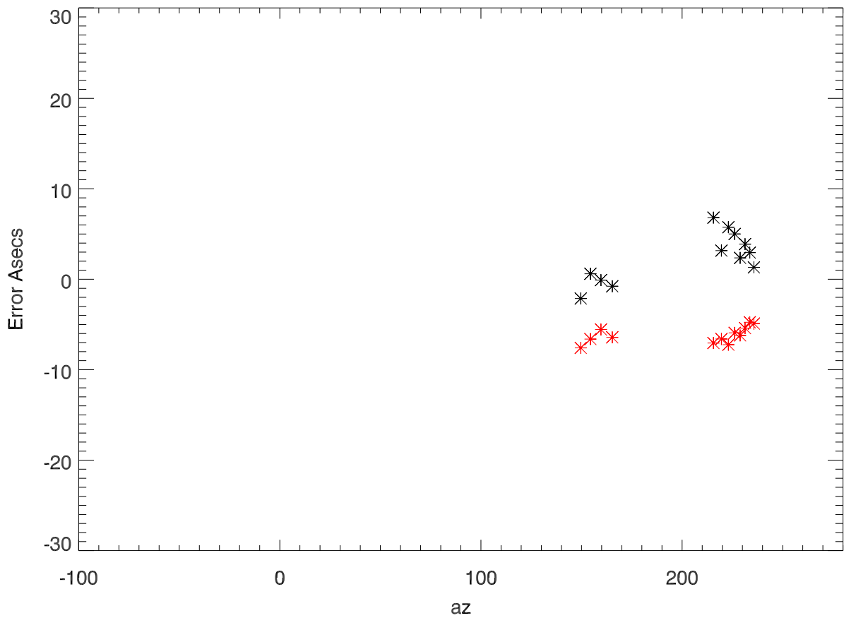
cross scan pointing err vs az 14jun10
