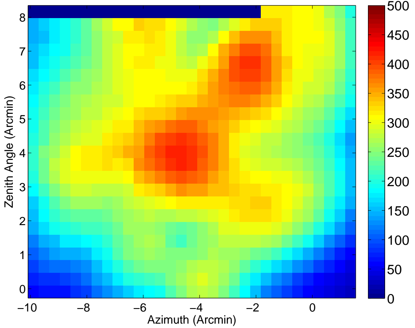
A1 Ae/Tsys Map ( z = 7.467 cm)
