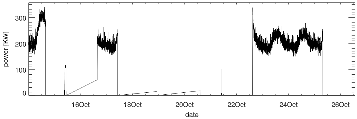
Total power vs Time (sum all generators)
