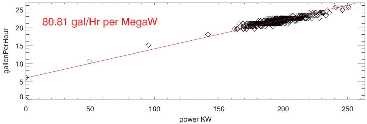
Fuel Rate vs power (sum all generators)
