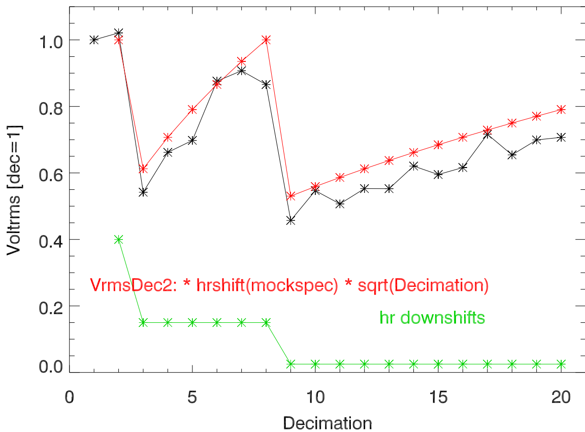
rmsvolts vs decimation normalized to dec=1
