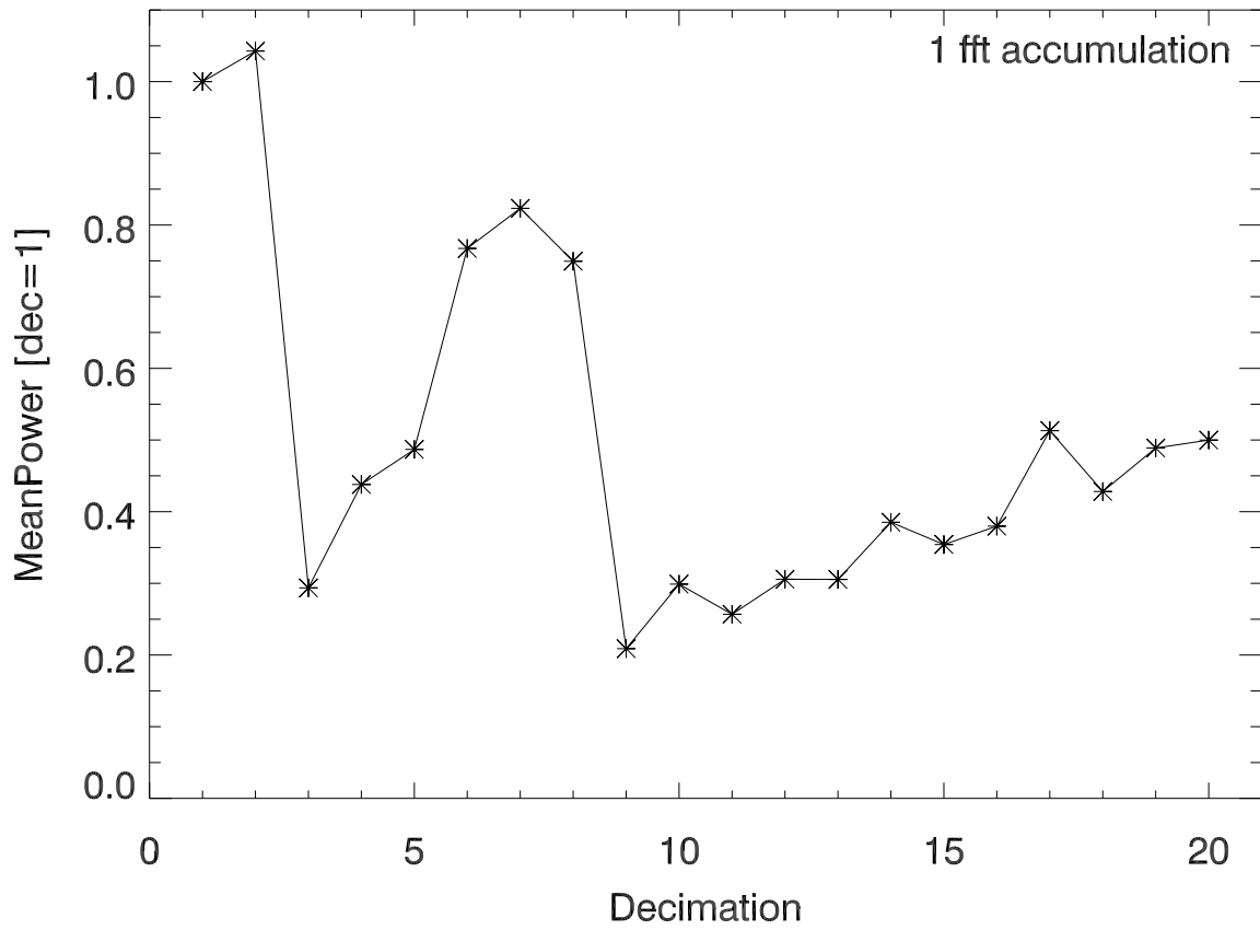
MeanPwr vs decimation normalized to dec=1
