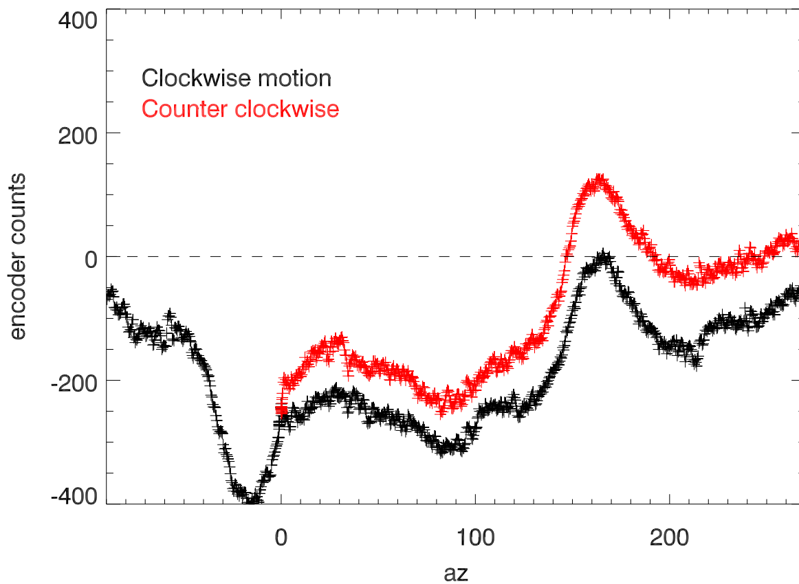
25nov11 az encoder difference after encoder 2 replaced
