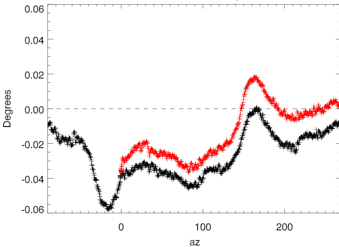
az encoder difference [Degrees] vs az
