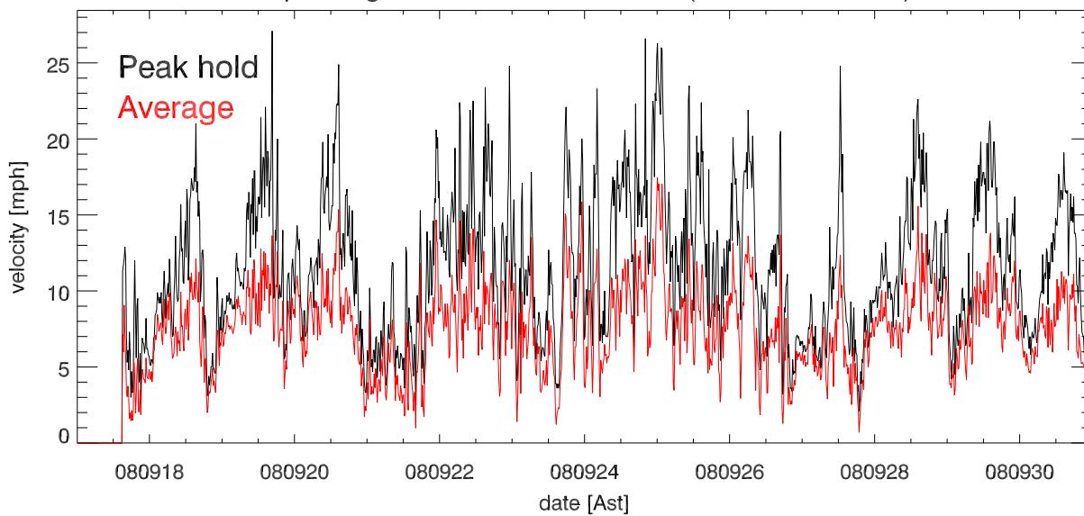
sep08 Avg & Peak velocities vs date (over 15.0 minutes)
