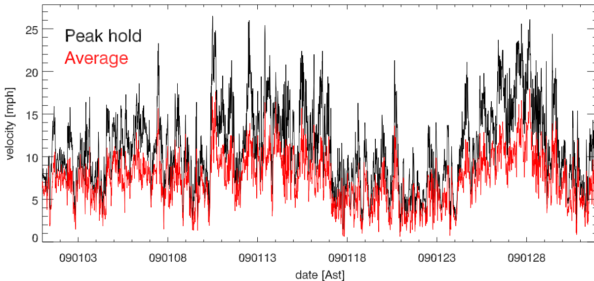
jan09 Avg & Peak velocities vs date (over 15.0 minutes)
