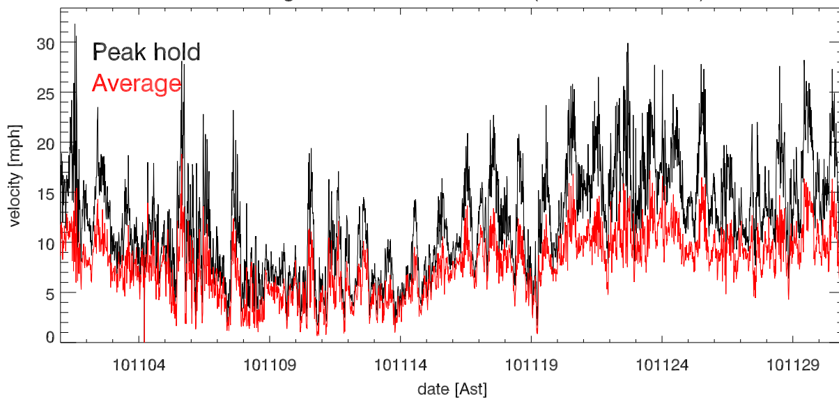
nov10 Avg & Peak velocities vs date (over 15.0 minutes)
