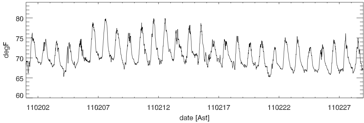
feb11 Temp vs date (averaged over 15.0 minutes)
