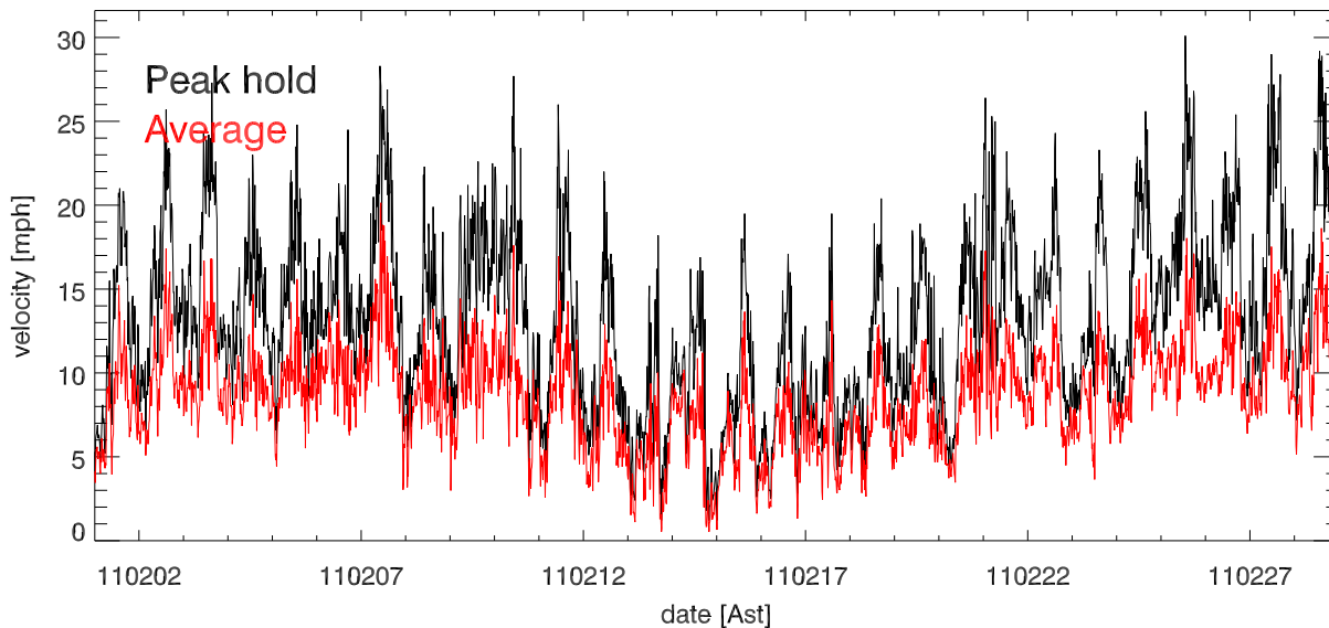
feb11 Avg & Peak velocities vs date (over 15.0 minutes)
