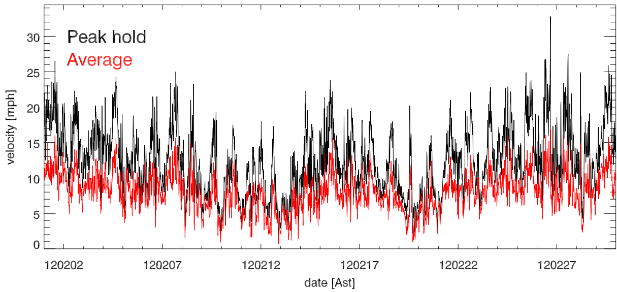
feb12 Avg & Peak velocities vs date (over 15.0 minutes)
