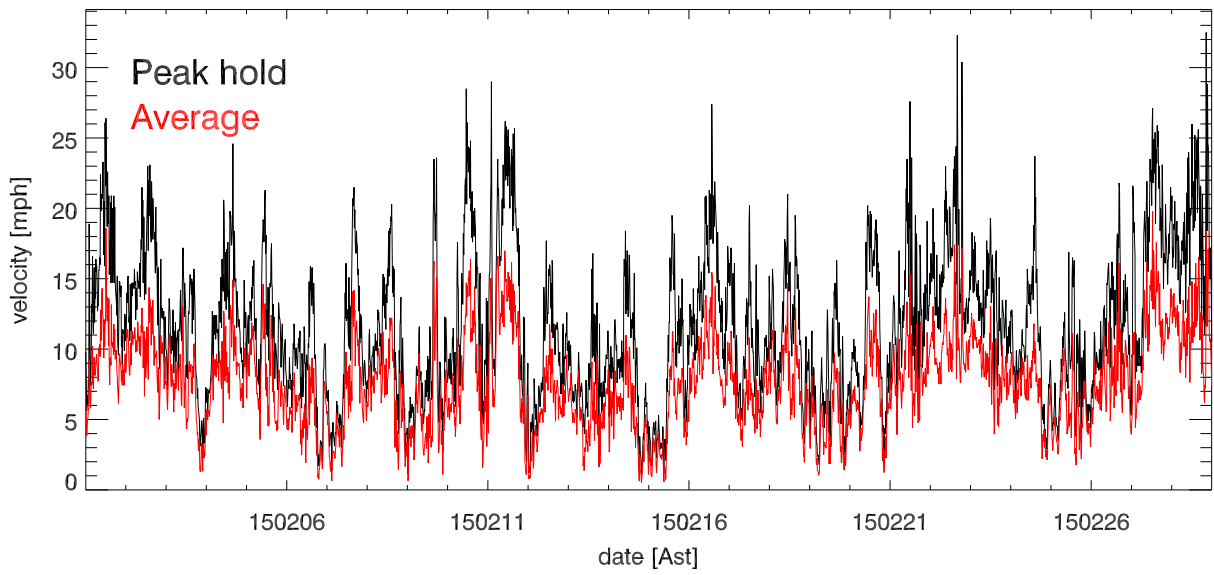
feb15 Avg & Peak velocities vs date (over 15.0 minutes)
