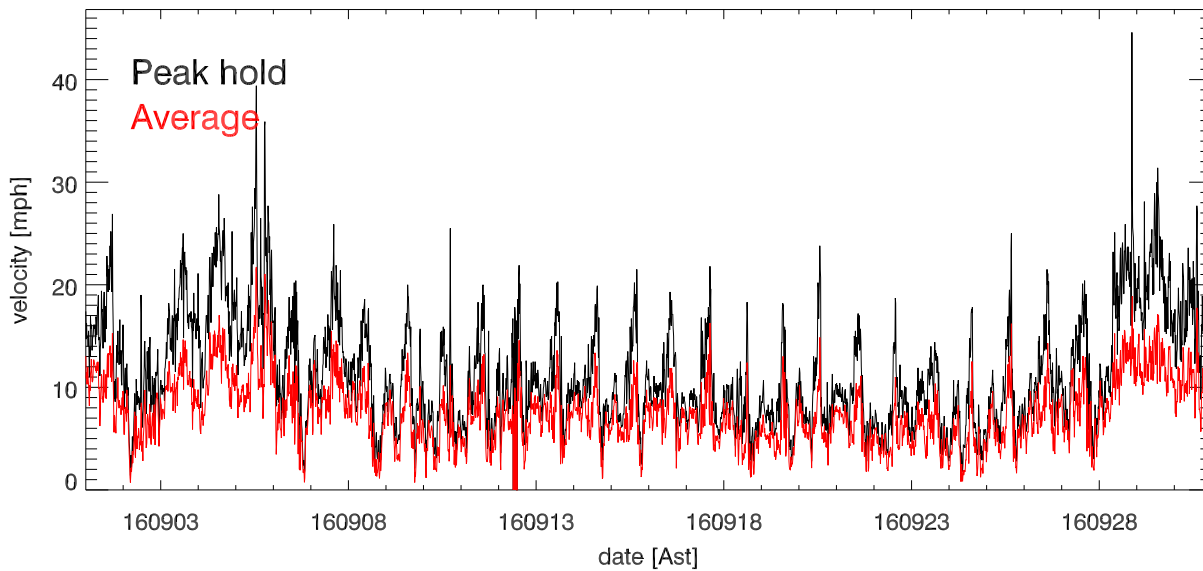
sep16 Avg & Peak velocities vs date (over 15.0 minutes)
