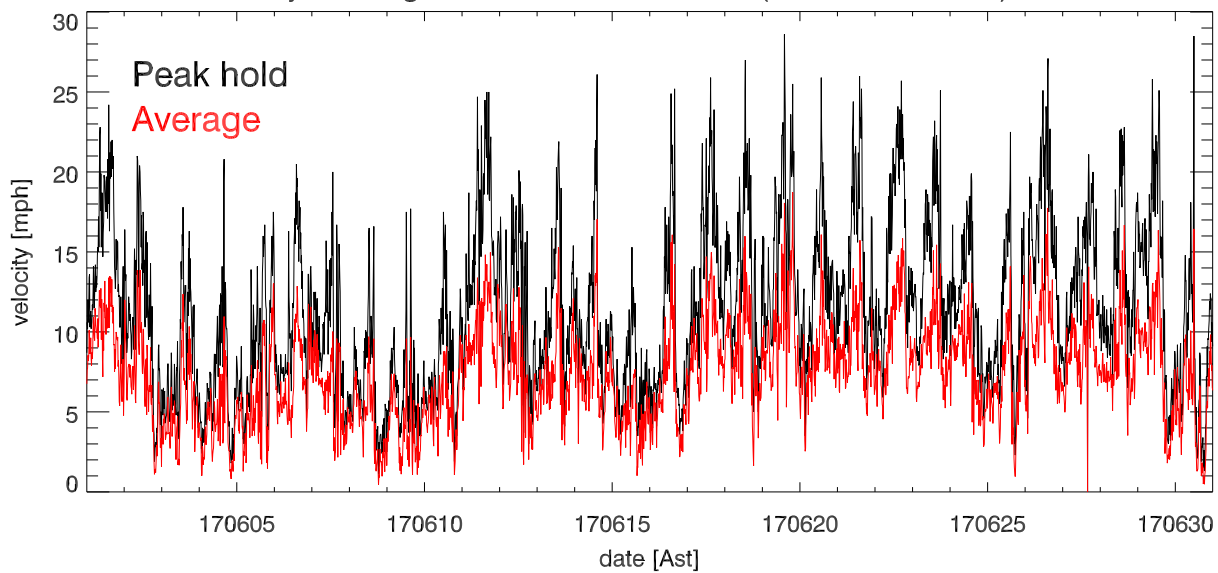
jun17 Avg & Peak velocities vs date (over 15.0 minutes)
