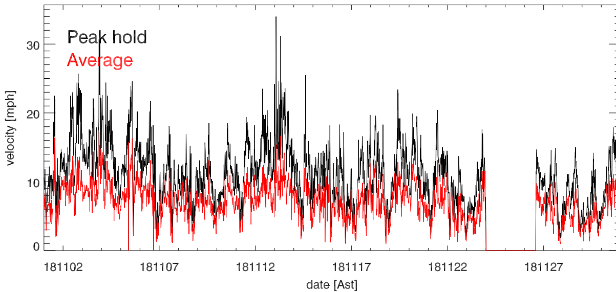
nov18 Avg & Peak velocities vs date (over 15.0 minutes)
