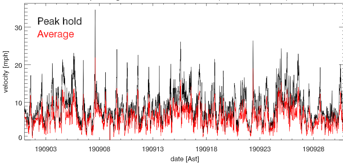
sep19 Avg & Peak velocities vs date (over 15.0 minutes)
