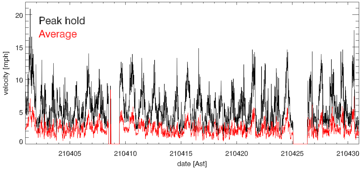
apr21 Avg & Peak velocities vs date (over 15.0 minutes)
