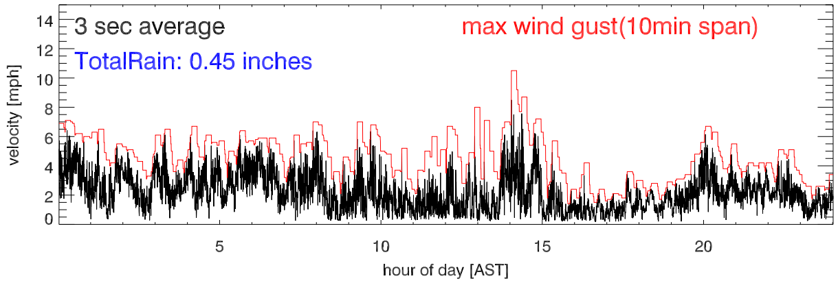
Wind velocity for 15oct21
