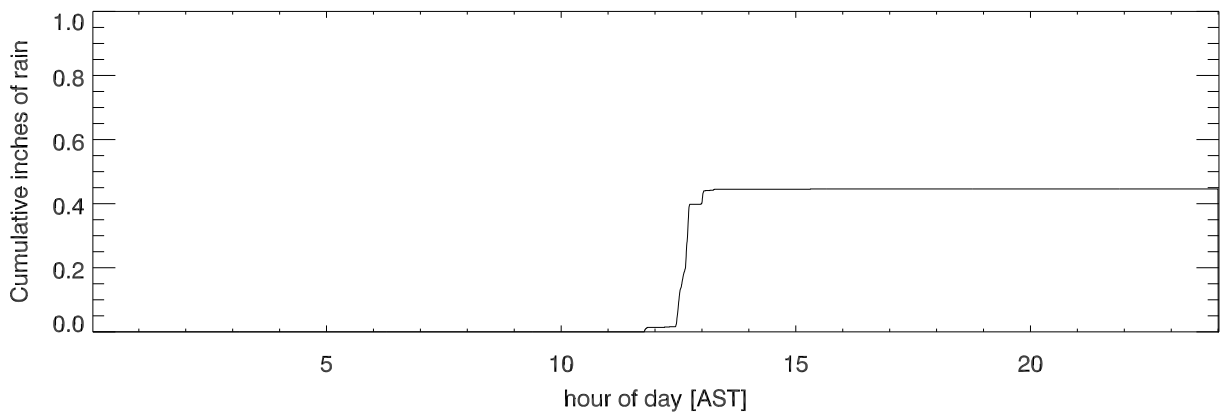
cumulative rain for 15oct21
