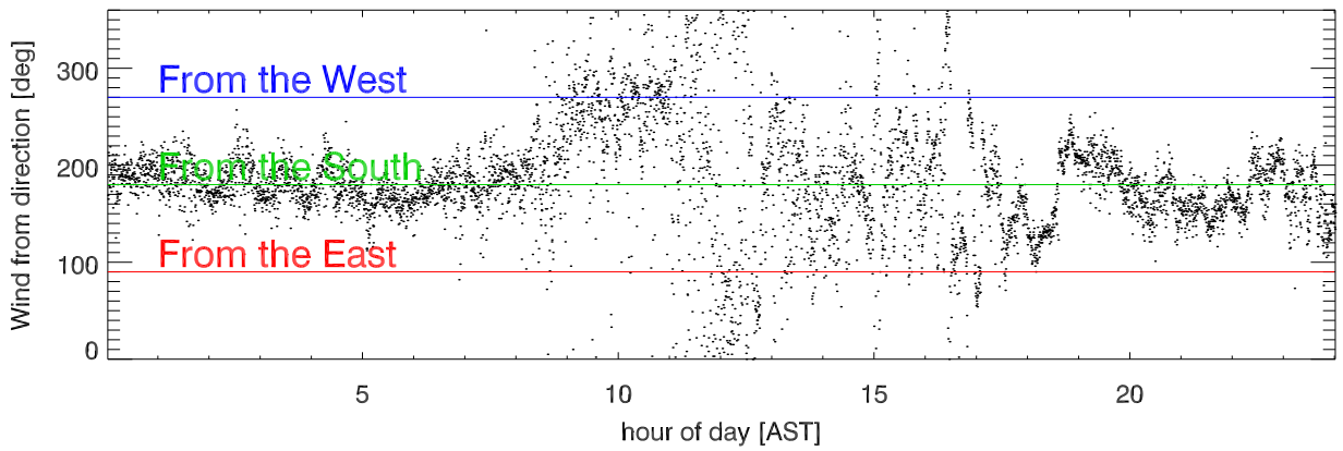
Wind direction for 15oct21
