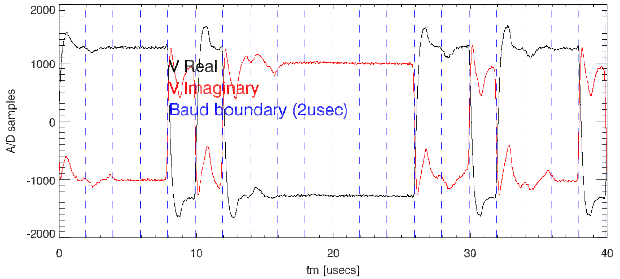
a3365 02oct19 12:48:01 USRP clp complex voltage during rf pulse
