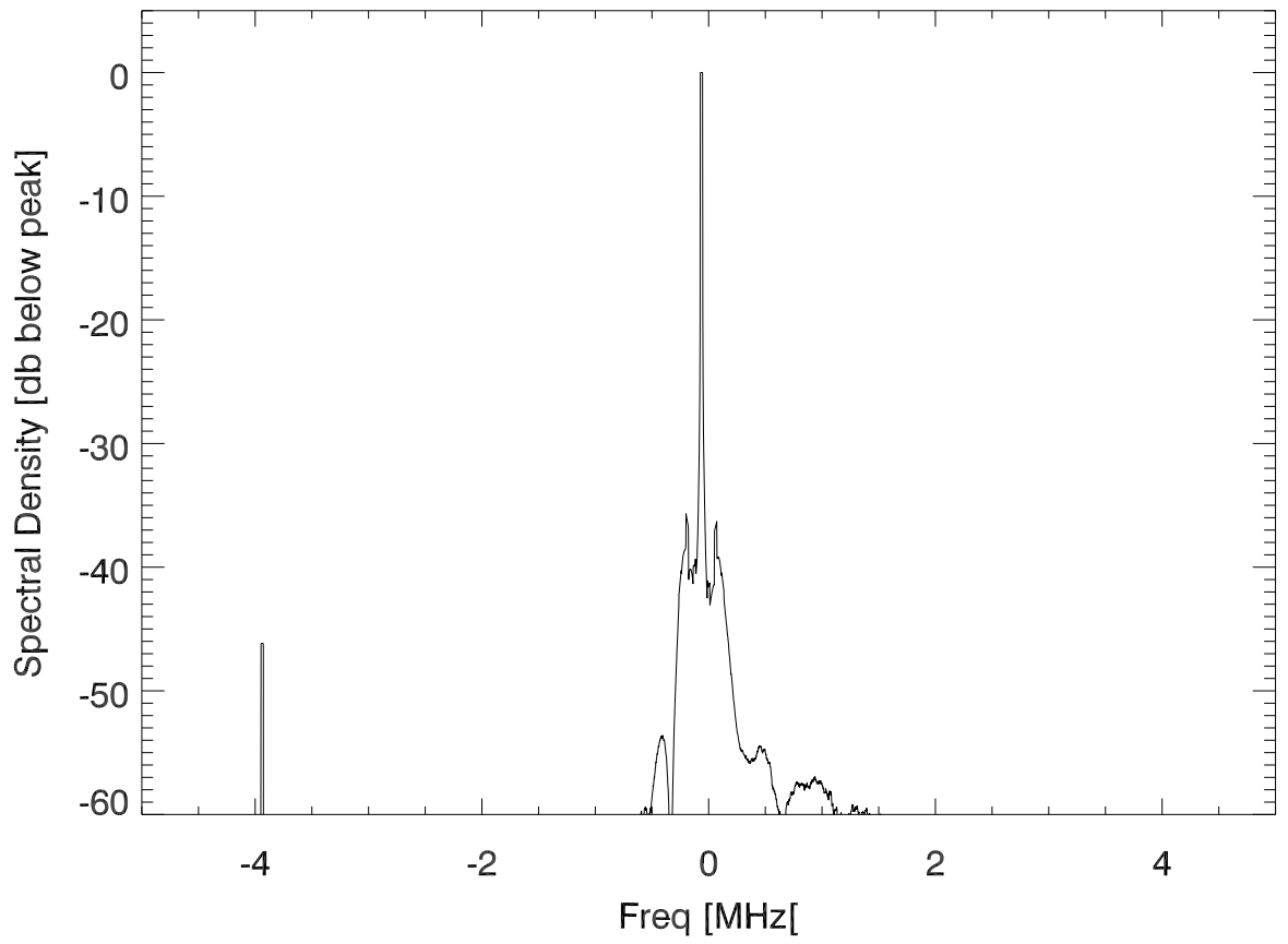
Spectral density of Tx tpsd rf pulse.
