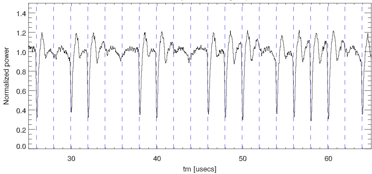
Normalized power during tx pulse
