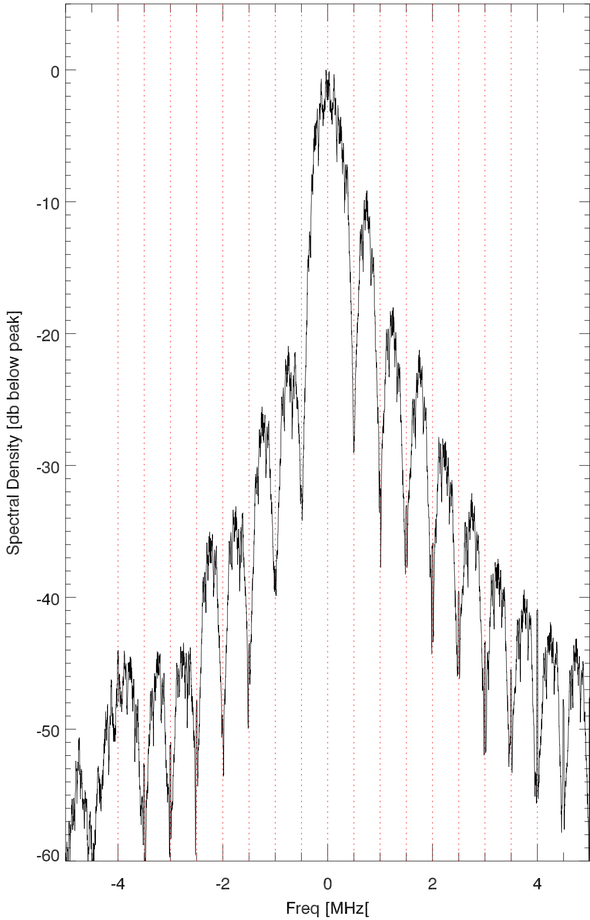
Spectral density of Tx clip rf pulse (baud=2usec)
