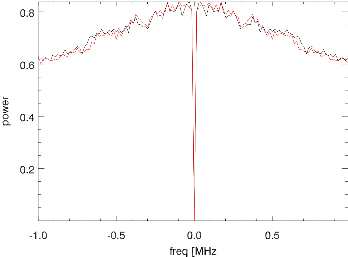
noise spectrum i,Q samples. avg 8000 ipp
