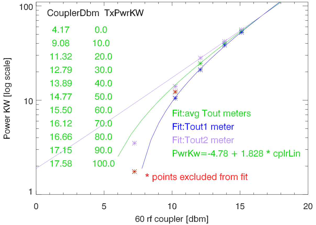
tx3 output power vs rf Coupler
