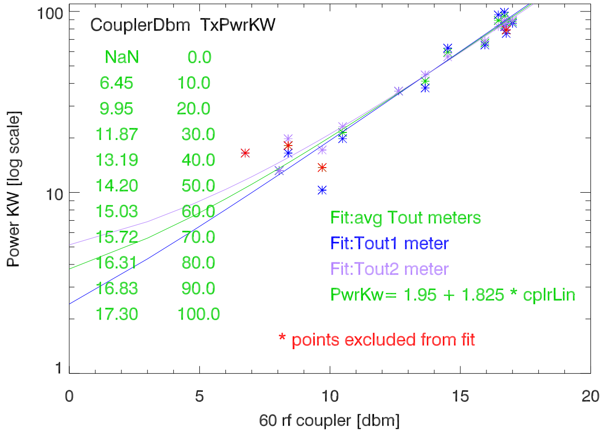
tx4 output power vs rf Coupler
