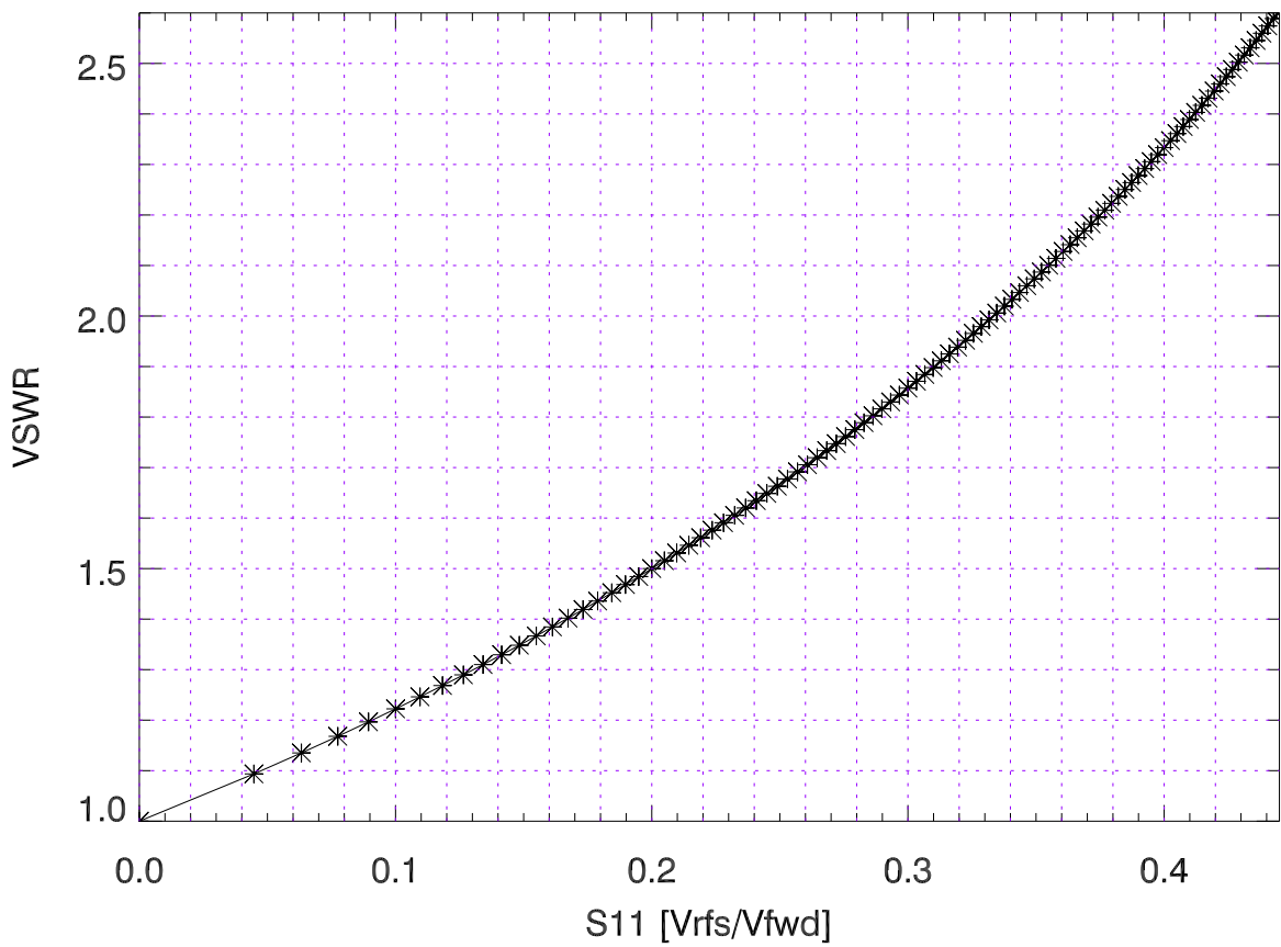
VSWR vs S11
