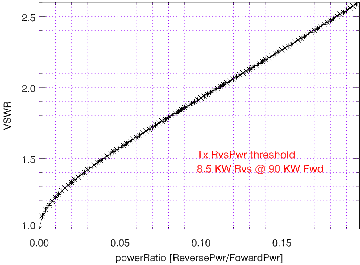
VSWR vs powerRatio (rvs/fwd)
