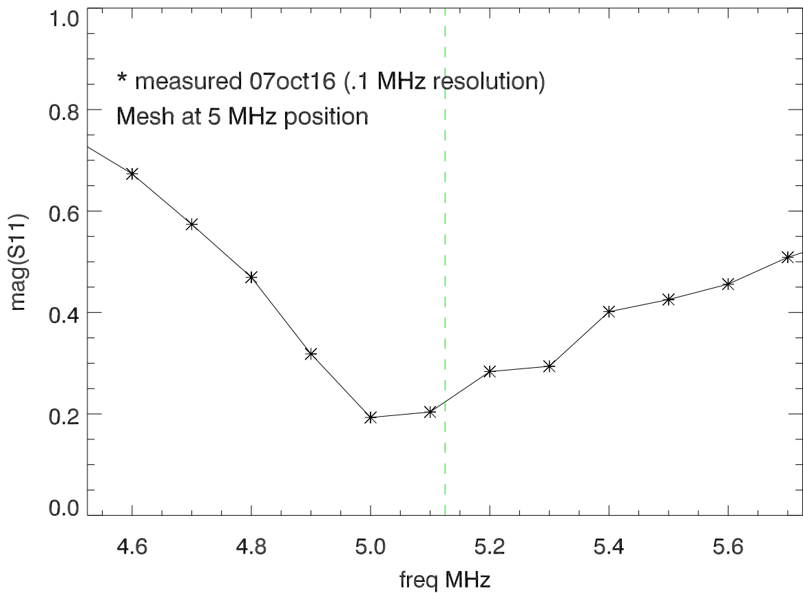
HF. mag(S11) vs freq. (Dipole 6B,tx6,5MHz).
