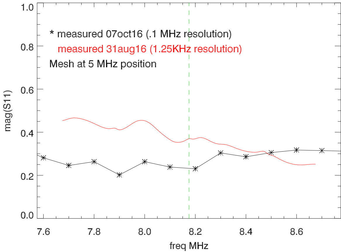
07oct16HF. mag(S11) vs freq. (Dipole 4b,tx4,8MHz).
