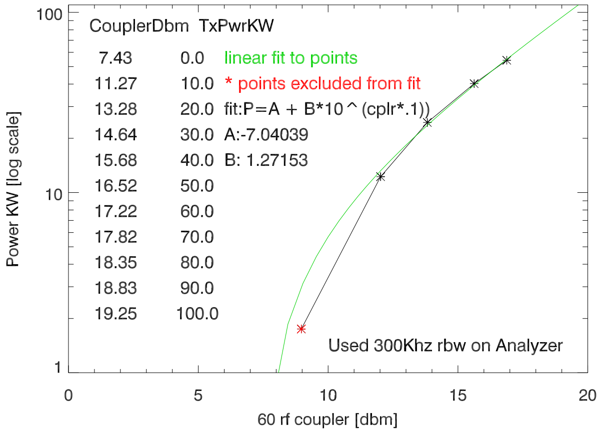
12may15 tx3 output power vs rf Coupler
