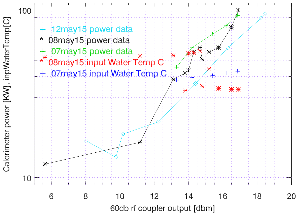
Tx4 output power vw rf Coupler:07,08,12may15
